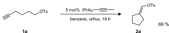
Scheme 2. Transformation of tosylate 1a in the presence of [IPrAu(propynyl)] ( 3a ; 5 mol %). Ts = tosyl = 4-toluenesulfonyl.
