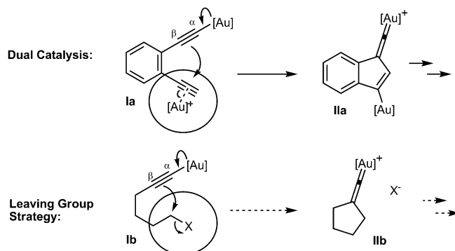
Scheme 1. Dual activation pathway leading to vinylidenes (top) and strategy for the synthesis of vinylidenes based on acetylides and a leaving group (bottom).
