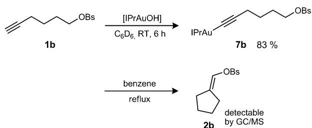
Scheme 3. Stoichiometric reaction of gold acetylide 7b .
