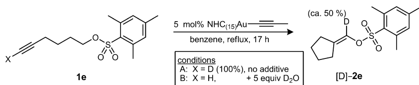
Scheme 4. Labeling experiments.
