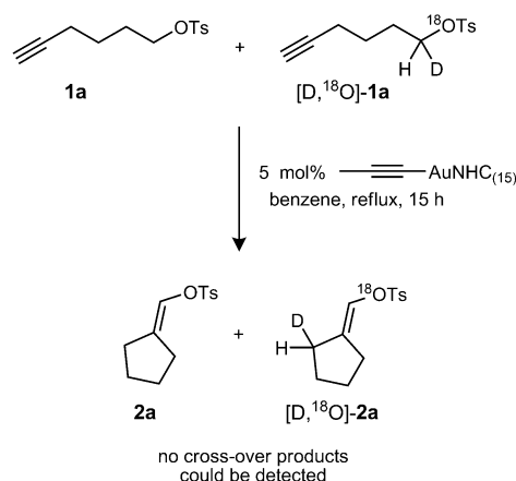
Scheme 5. Cross-over experiment.
