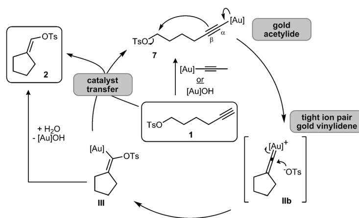
Scheme 6. Proposed reaction mechanism. OTs is used as a representative for the sulfonate leaving groups.
